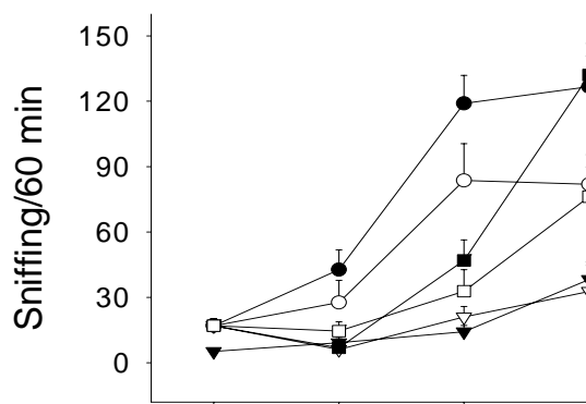
Apomorphine (mg/kg)
